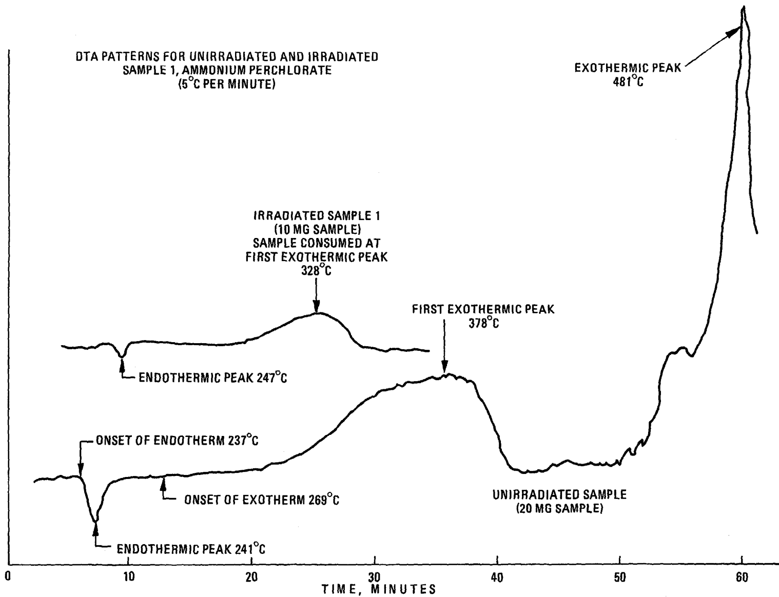
Fig 21 DTA of Ammonium Perchlorate Showing Effect of Reactor Irradiation ( 10^7 n/cm 2 , 1.7 \times 10^8 R) (Ref 177)
